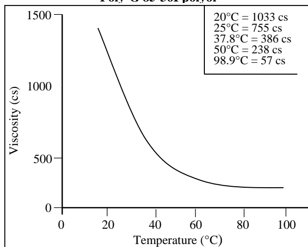
Figure 1 Viscosity vs. Temperature Poly-G 85-36I polyol
