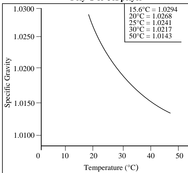
Figure 2 Specific Gravity vs. Temperature Poly-G 85-36I polyol
