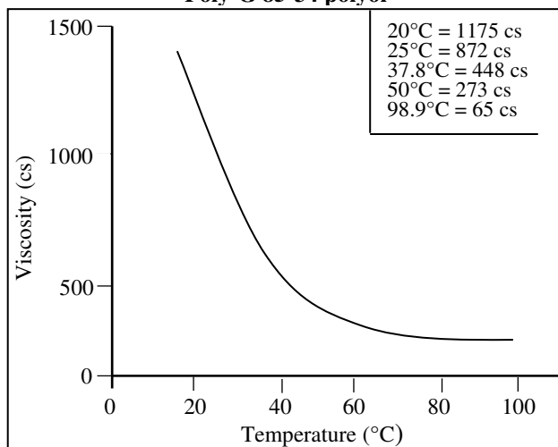
Figure 1 Viscosity vs. Temperature Poly-G 85-34 polyol
