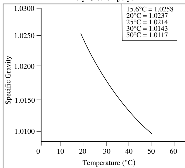
Figure 2 Specific Gravity vs. Temperature Poly-G 85-34 polyol
