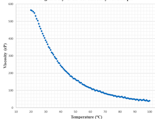
Fig. 1 Poly-G 83-65 Viscosity vs. Tempt.
