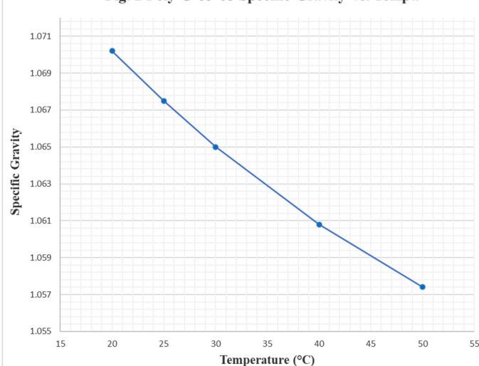
Fig. 2 Poly-G 83-65 Specific Gravity vs. Tempt.
