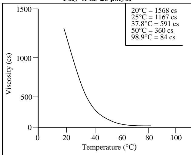
Figure 1 Viscosity vs. Temperature Poly-G 83-26 polyol
