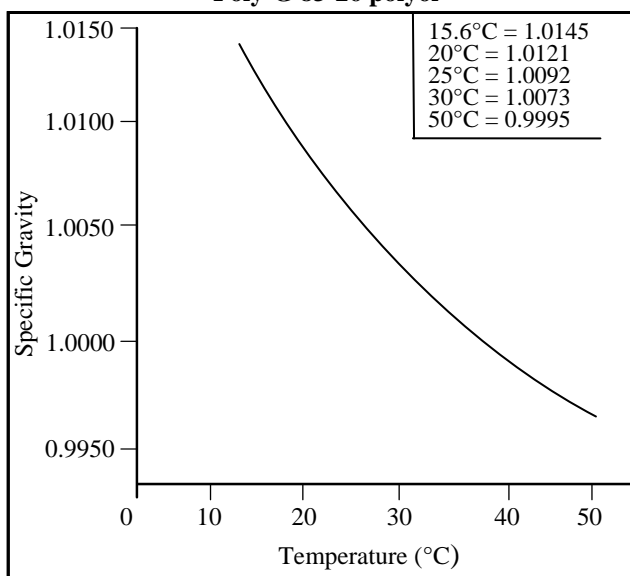
Figure 2 Specific Gravity vs. Temperature Poly-G 83-26 polyol
