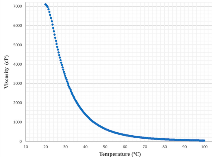
Fig. 1 Poly-G 74-380 Viscosity vs. Tempt.
