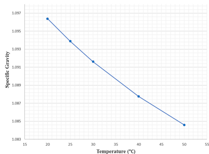
Fig. 2 Poly-G 74-380 Specific Gravity vs. Tempt.
