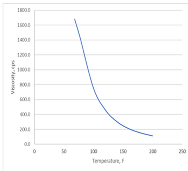
Figure 1 Viscosity vs. Temperature Poly-Q 53-35
