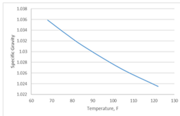
Figure 2 Specific Gravity vs. Temperature Poly-Q 53-35
