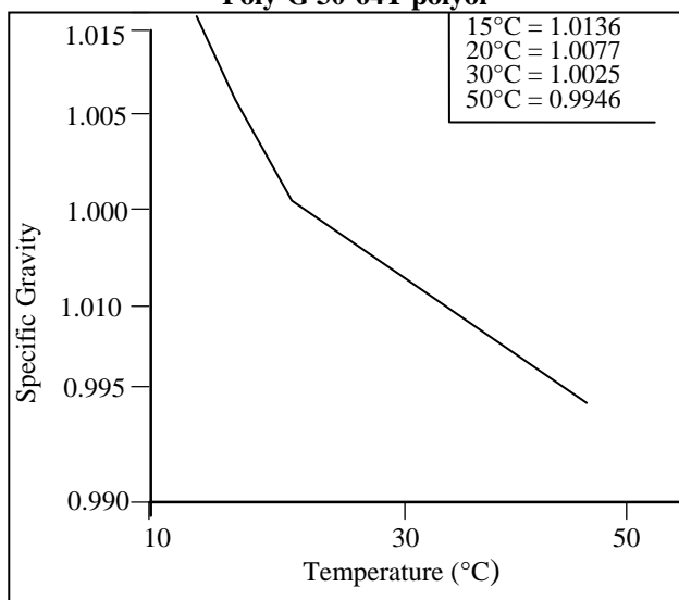
Figure 2 Specific Gravity vs. Temperature Poly-G 30-64T polyol
