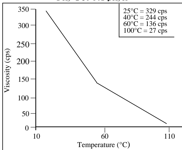
Figure 1 Viscosity vs. Temperature Poly-G 30-64T polyol
