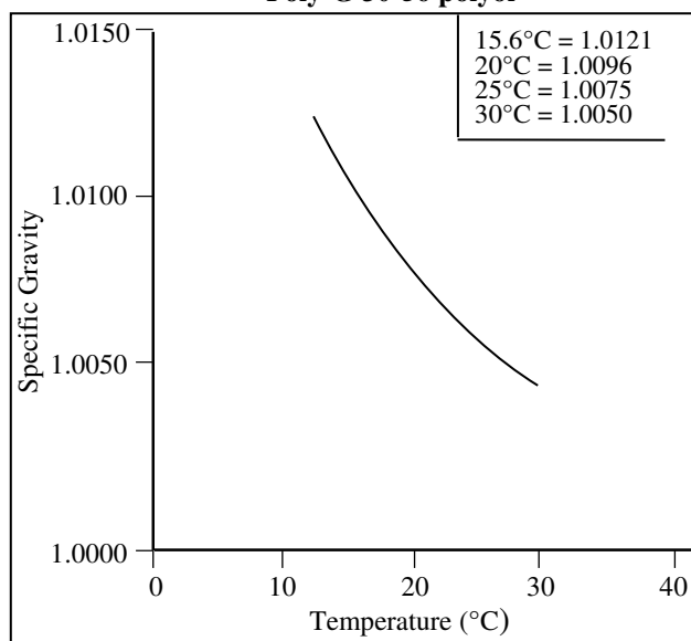
Figure 2 Specific Gravity vs. Temperature Poly-G 30-56 polyol
