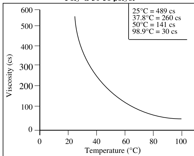
Figure 1 Viscosity vs. Temperature Poly-G 30-56 polyol
