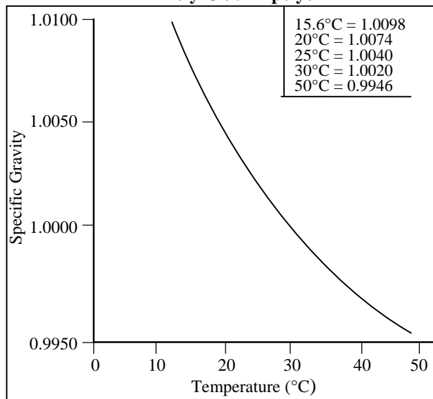
Figure 2 Specific Gravity vs. Temperature Poly-G 30-42 polyol
