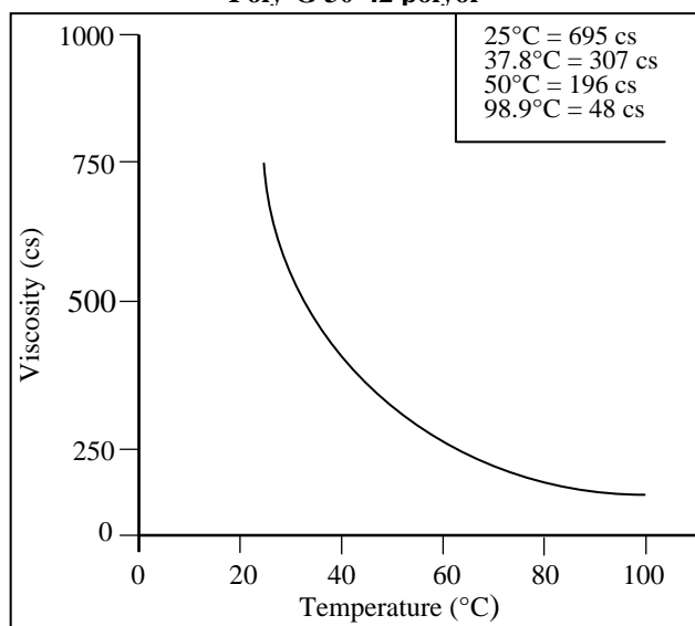
Figure 1 Viscosity vs. Temperature Poly-G 30-42 polyol
