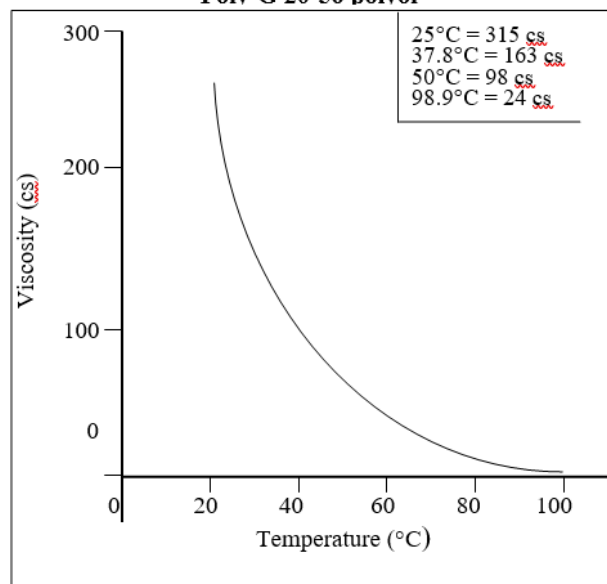
Figure 1 Viscosity vs. Temperature Poly-G 20-56 polyol
