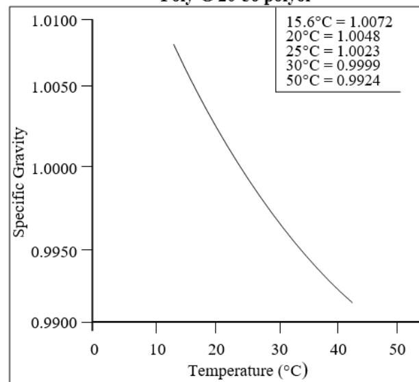
Figure 2 Specific Gravity vs. Temperature Poly-G 20-56 polyol
